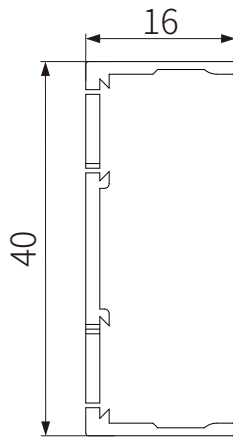
Vertical Cover
